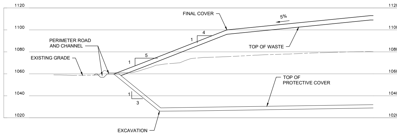
D FINAL COVER SECTION HIL-A-89 HORIZ 0 50 100 VERT 0 5 10 SCALE IN FEET
