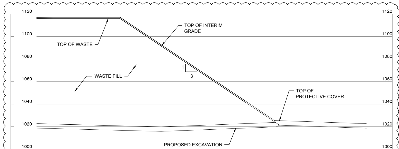
F INTERIM SECTION HIL-A-89 HORIZ 0 50 100 VERT 0 5 10 SCALE IN FEET
