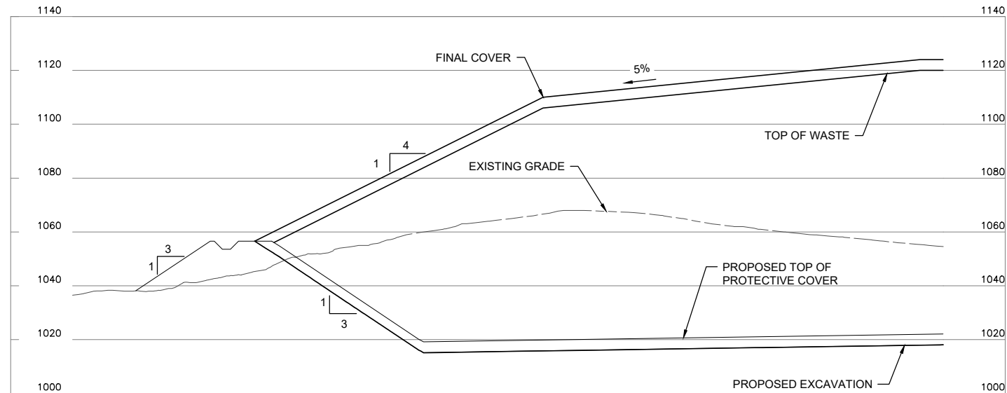
C FINAL COVER SECTION HIL-A-89 HORIZ 0 50 100 VERT 0 5 10 SCALE IN FEET
