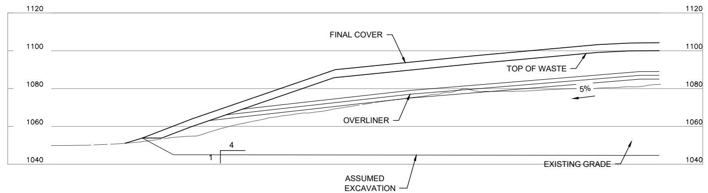
E OVERLINER HIL-A-89 HORIZ 0 50 100 VERT 0 5 10 SCALE IN FEET
